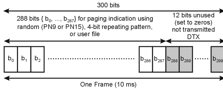
Figure 4-1. PICH Frame Structure
